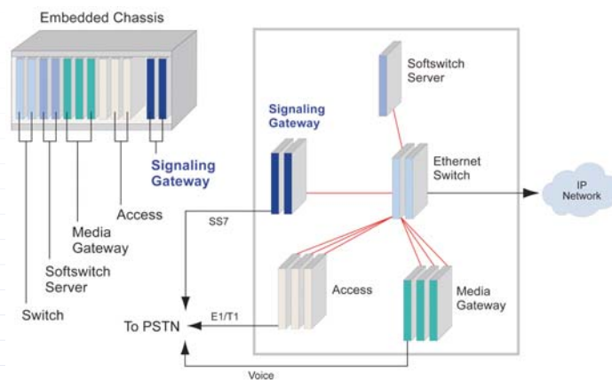
The Signaling Gateway 5601 in an Embedded VoIP Architecture Environment
